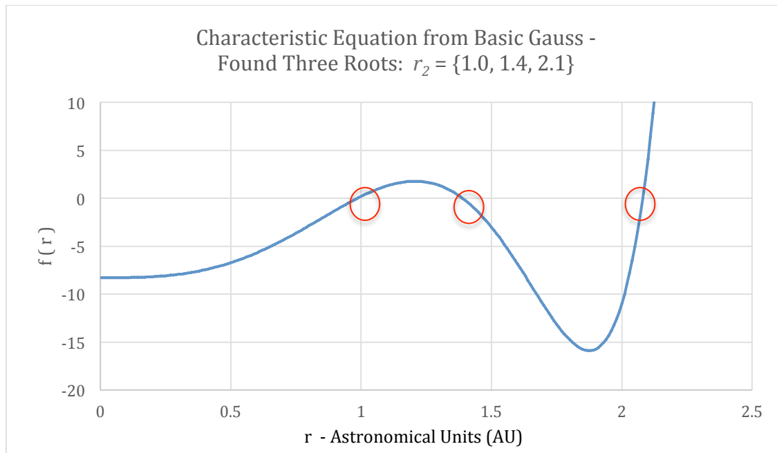
Figure 6: Plot of a representative characteristic equation
