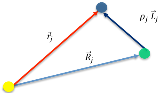
Figure A.2: Line of sight vector and Earth and Comet position vectors at time t_j .
