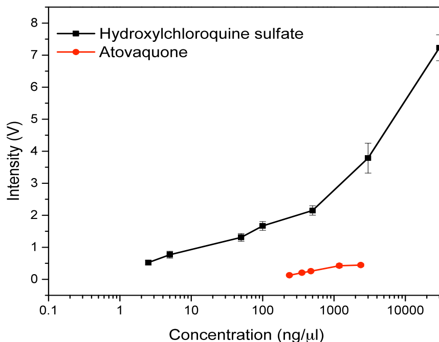
Figure 7. Response curves. The response curves are limited to low nanogram when in theory and practice, response should be observed in the low picogram. This is attributed to poor design and operation of ion source and electric fields in the source region.
