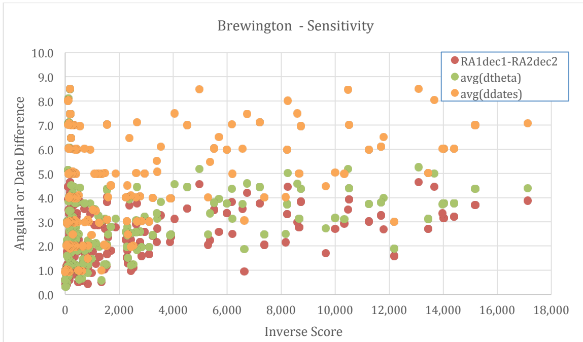
Figure 13: Sensitivity of Brewington orbital elements to date and angular spacing
