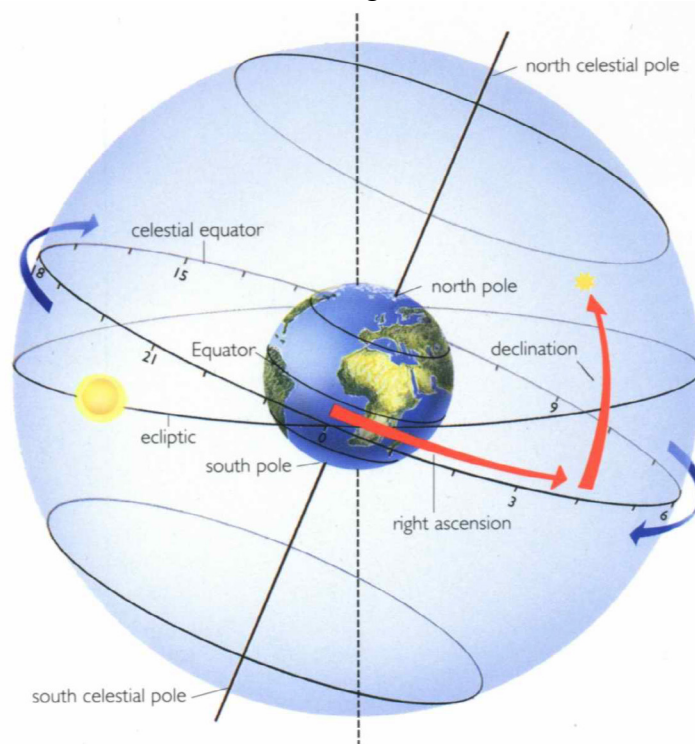
Figure 2: Equatorial coordinate system – showing the right ascension and declination angles and the ecliptic and equatorial planes (source: http://crab0.astr.nthu.edu.tw/~hchang/ga1/f0202-equatorial.JPG )
