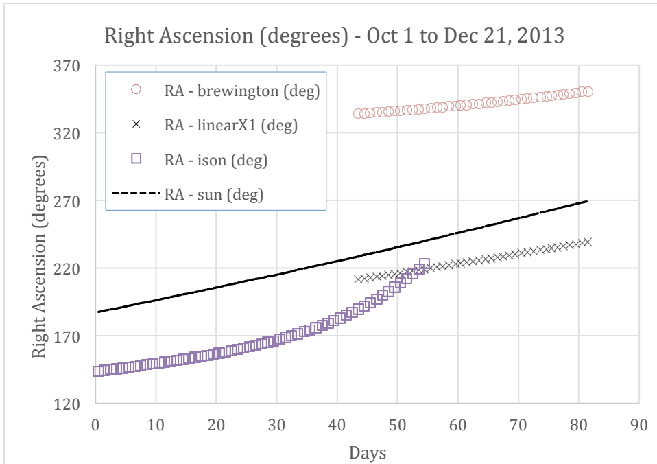
Figure 4: Right ascension input data
