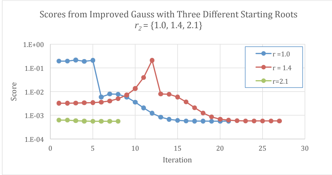
Figure 7: Representative example of iteration with the Improved Gauss routine
