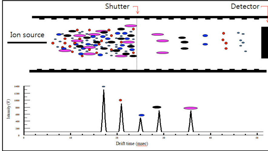
Figure 1. Mobility of Ions in Electric Fields (Up. ions in drift tube with electric field, Down. Spectrum obtain from mobility analysis)
