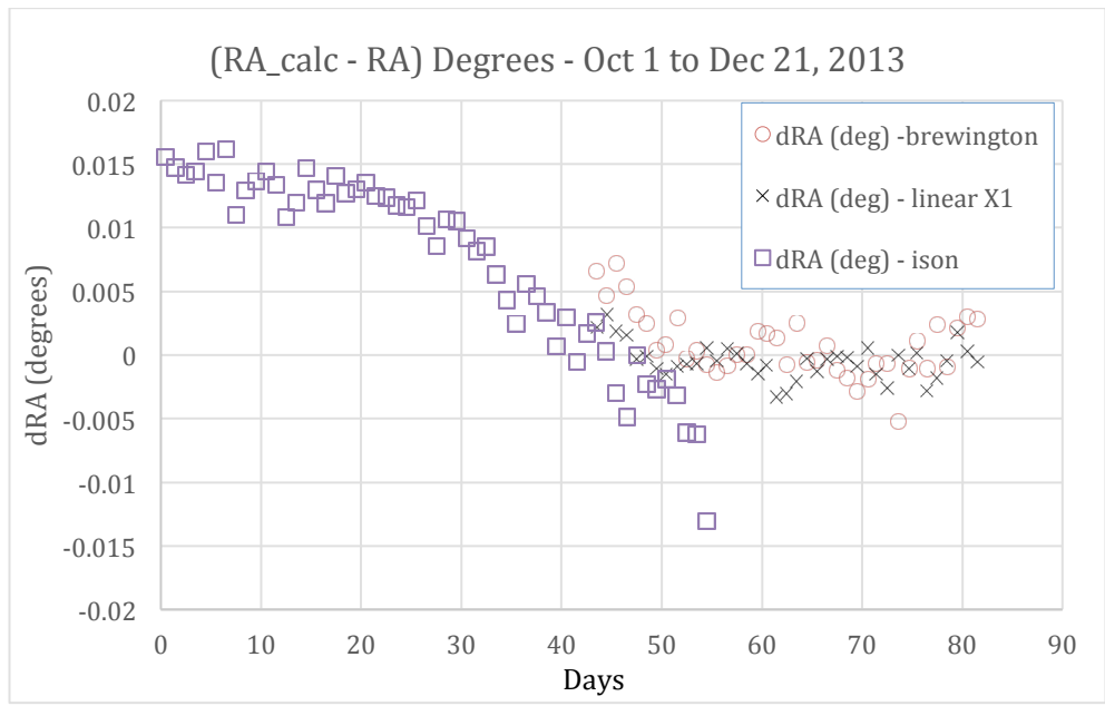
Figure 11: Error in daily right ascension using best sets of elements
