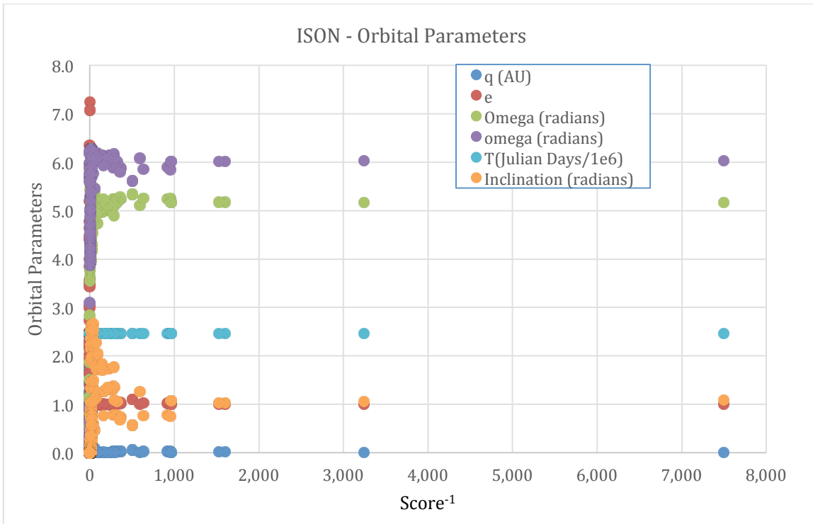
Figure 10: ISON orbital elements vs. inverse score
