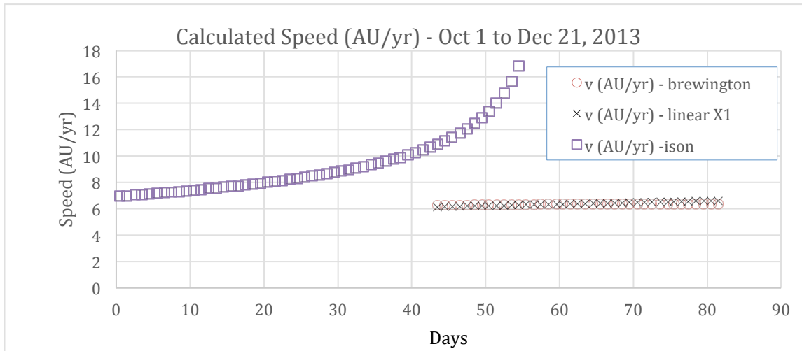
Figure 16: Calculated speed using the lowest-score orbital elements
