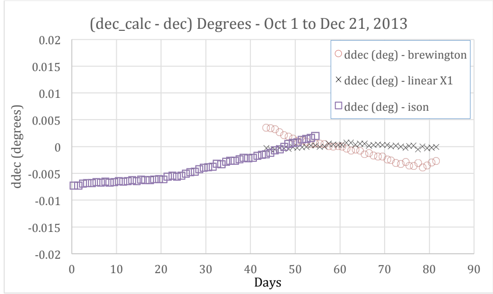
Figure 12: Error in daily declination using best sets of elements
