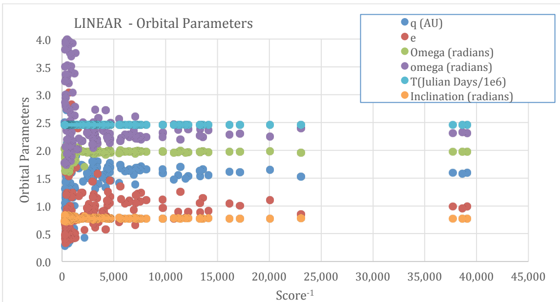
Figure 9: LINEAR orbital elements vs. inverse score
