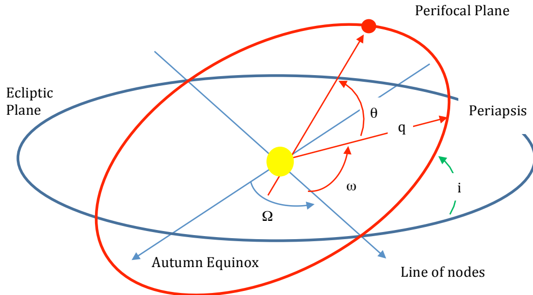
Figure 1: Classical orbital elements
