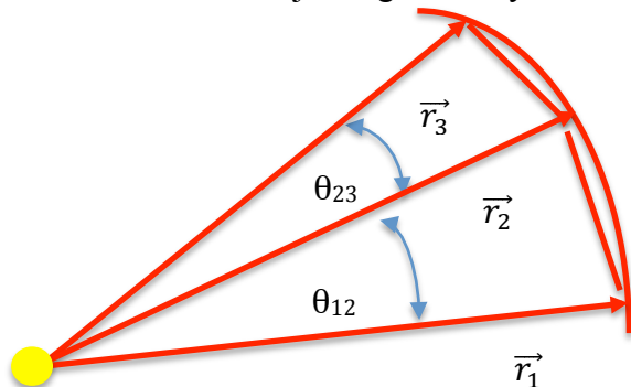
Figure A.3: Comet position vectors at 3 times
