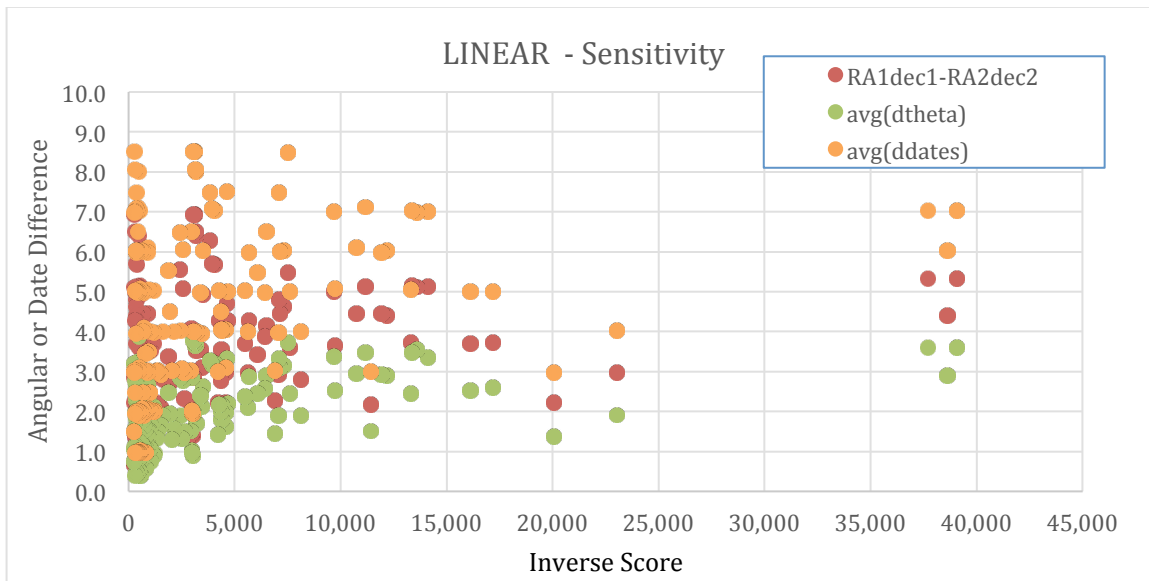
Figure 14: Sensitivity of LINEAR orbital elements to date and angular spacing
