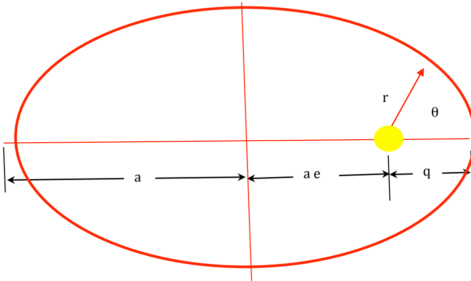
Figure A.1: Perifocal coordinates and the conic properties.
