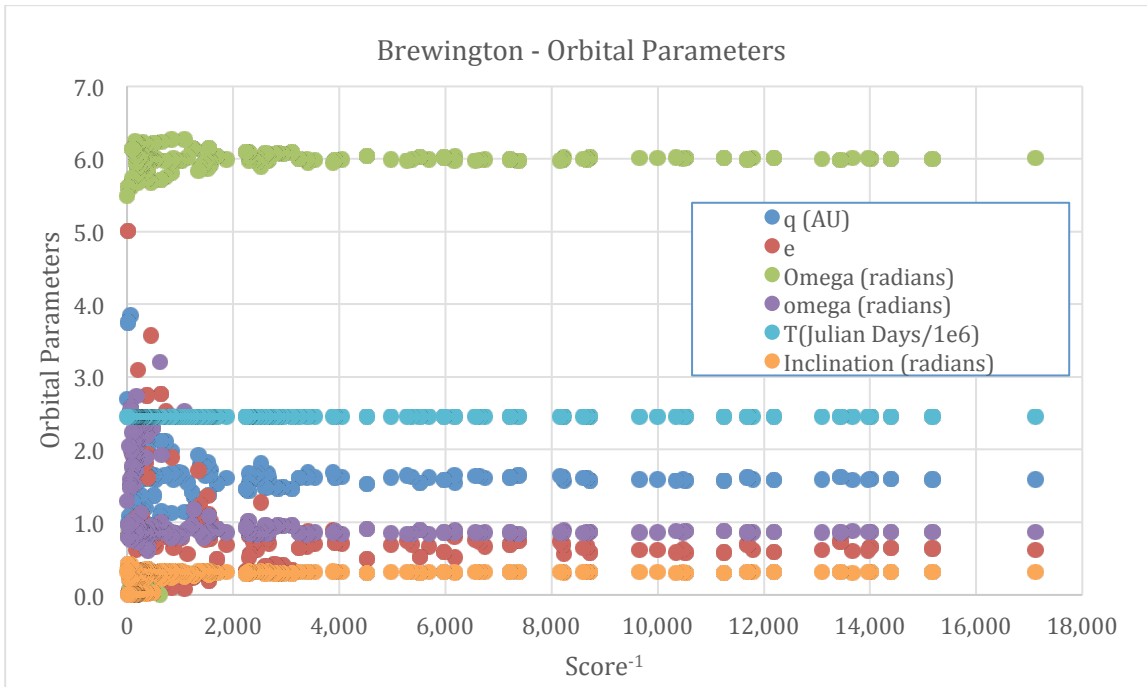
Figure 8: Brewington orbital elements vs. the inverse score
