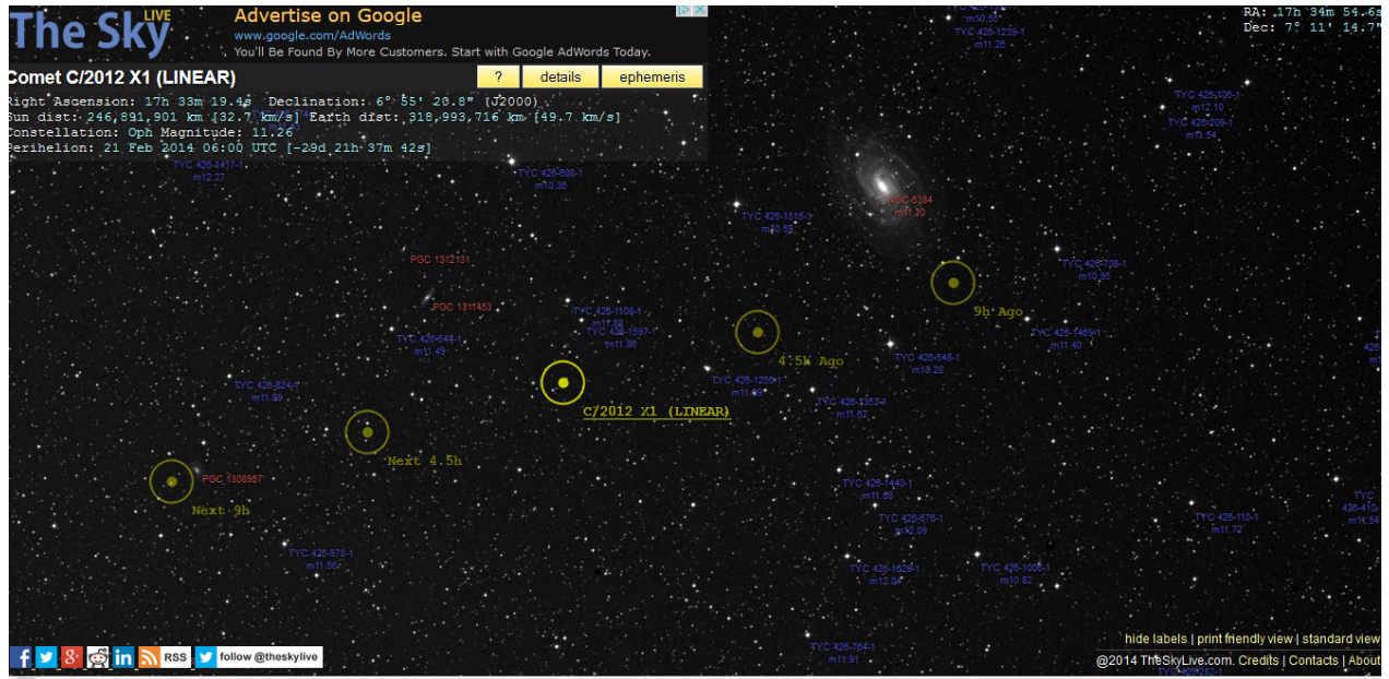
Figure 3: Representative data from theskylive.com
