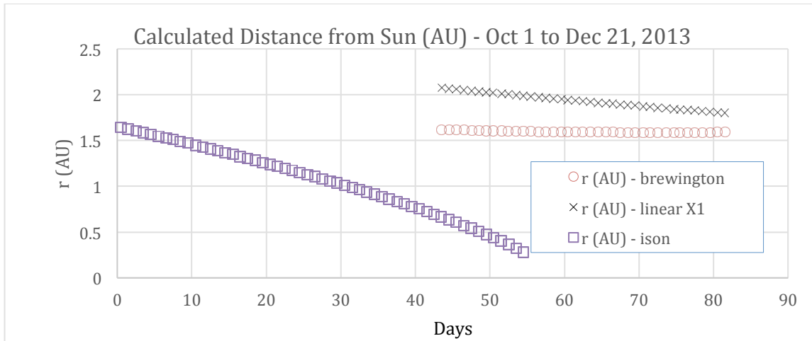
Figure 15: Calculated distance from Sun, using the lowest-score orbital elements
