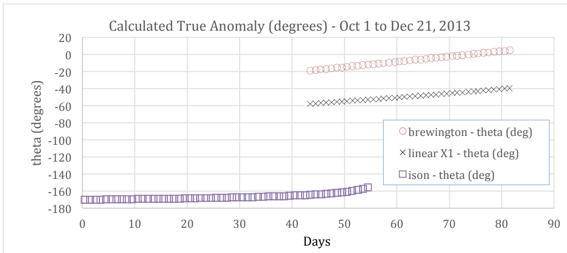
Figure 17: Calculated true anomaly using the lowest-score orbital elements
