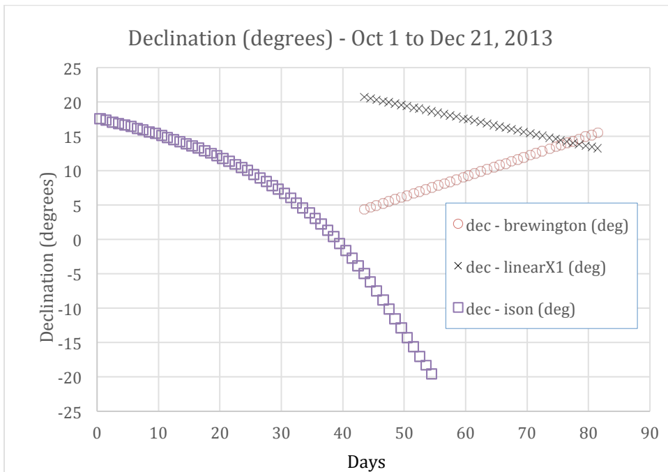
Figure 5: Declination input data
